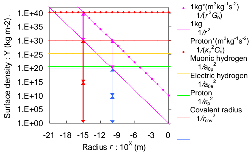
Fig. 1. Ratios among quantum size, nuclear force and gravity
