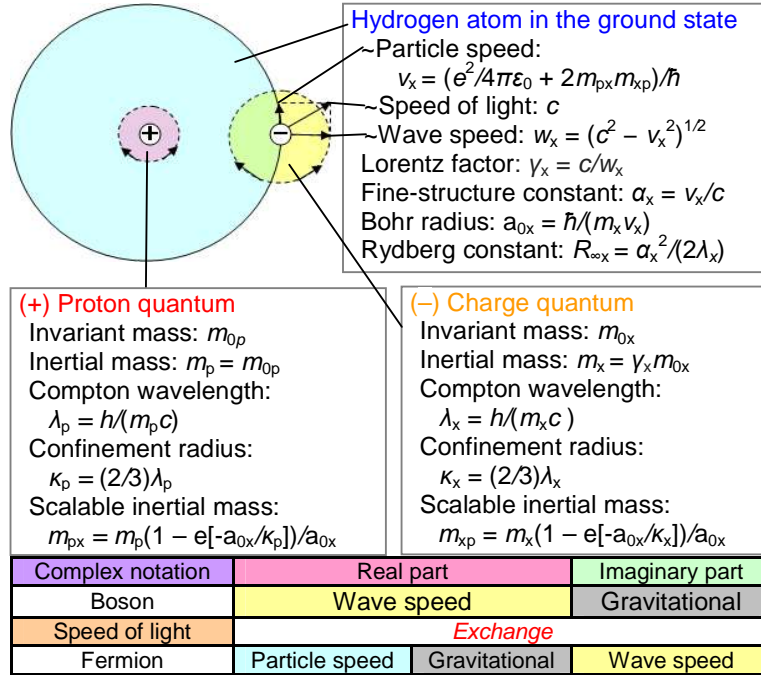
Fig. 2. Model of the internal relationships among the structures of a ground-state hydrogen atom
