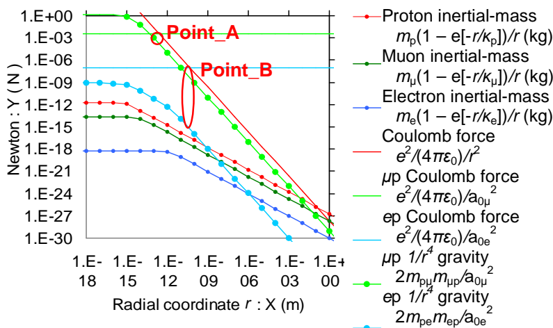
Fig. 3. The scalable inertial mass of fermions and the coulomb force and the 1/r^4 gravity of a combination thereof
