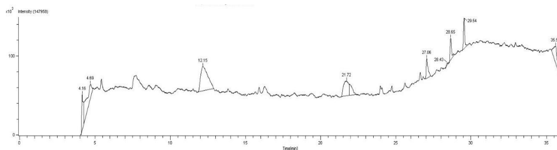
Fig. 1. Gas chromatography mass spectrometry graph of compounds identified in methanolic extract of Juglans regia shells
