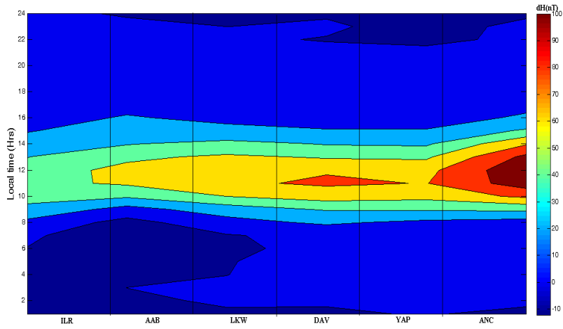
Fig. 3. dH during E-season
