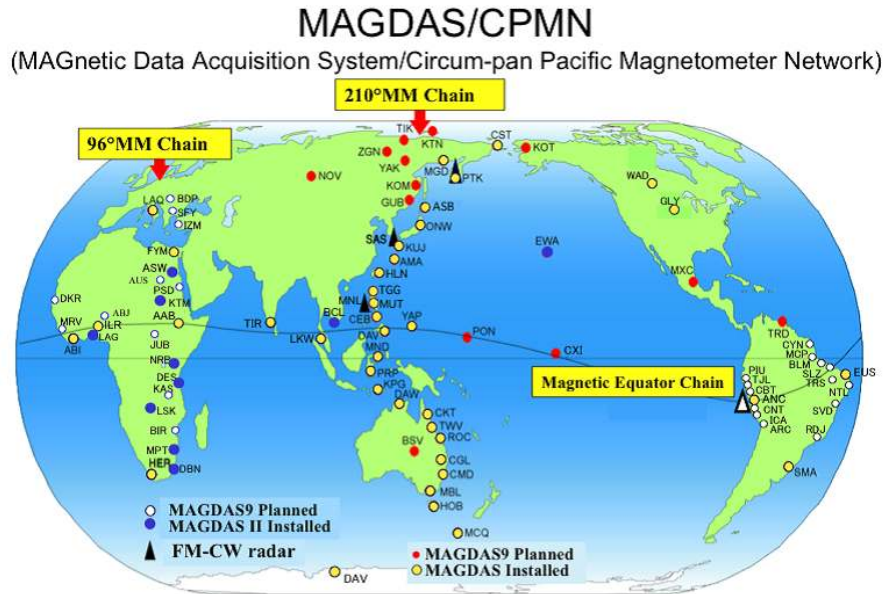
Fig. 1. The global network of MAGDAS magnetometers
