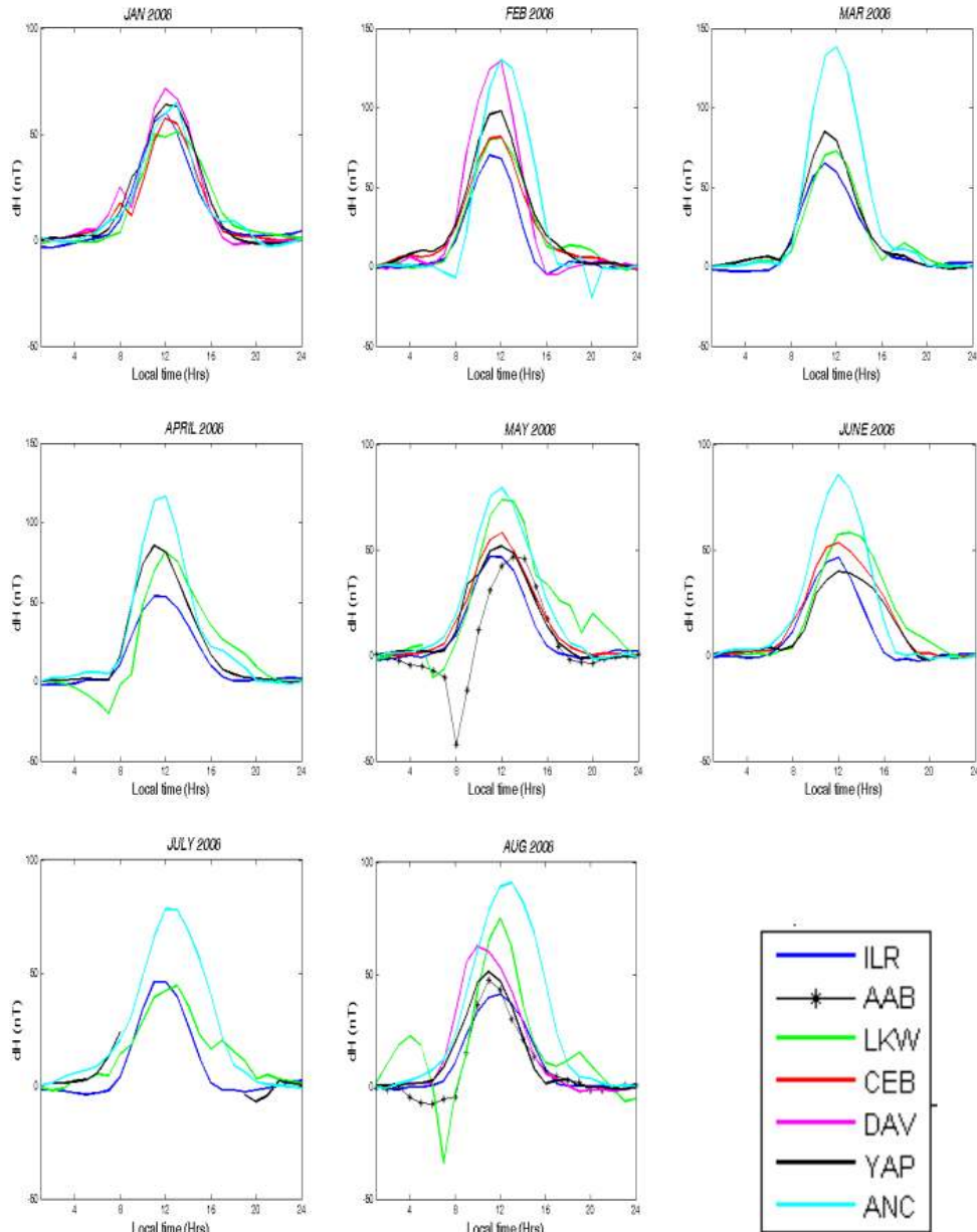
Fig. 2. Monthly mean daily variations of H field for five international quiet days
