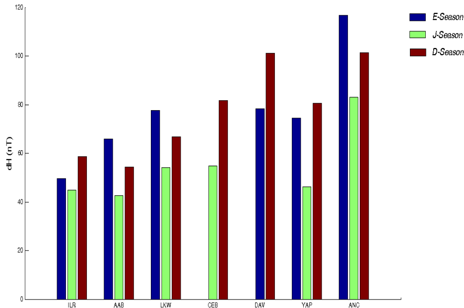
Fig. 6. Seasonal variation of noon-time dH across the stations
