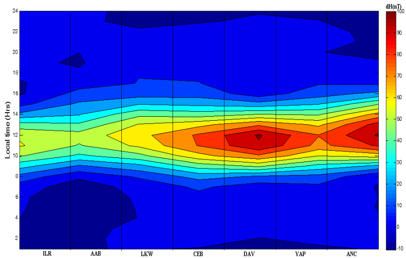
Fig. 5. dH during D-season
