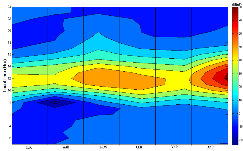
Fig. 4. dH during J-season
