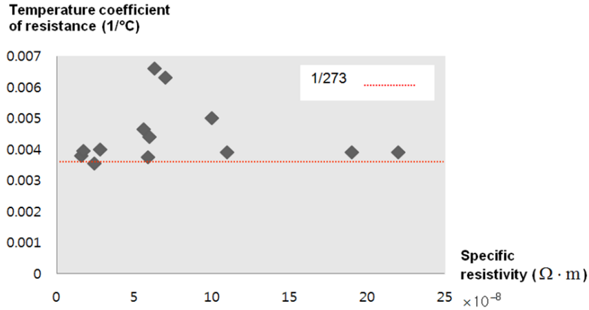
Fig. 1. The scatter diagram of the temperature coefficients of resistance of the good conductors in Table 1 compared with the temperature coefficient, 1/273, in Charles’s law
