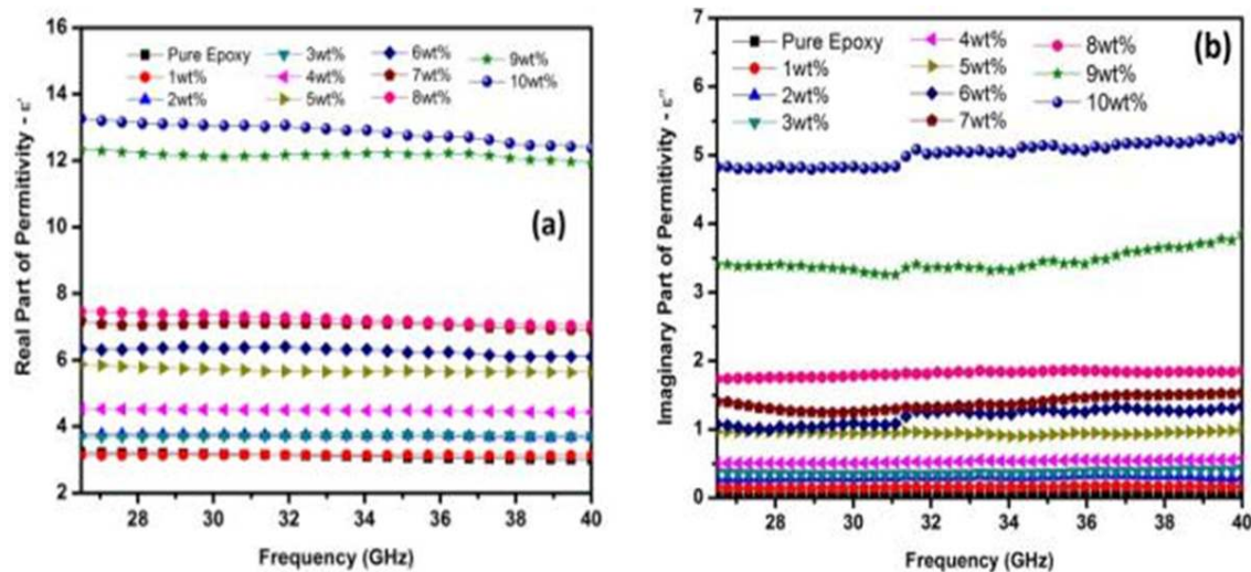
Fig. 3. Real part ( \epsilon' ) and Imaginary part ( \epsilon'' ) of relative dielectric permittivity of pure epoxy and MWCNTs-epoxy composites with MWCNT loading fractions from 1 – 10 wt.%
