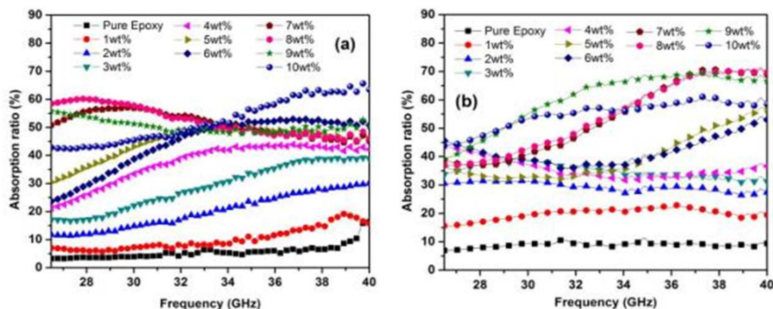
Fig. 5. Absorption ratio (in %) of (a) 2 mm and (b) 3 mm pure epoxy and MWCNTs-epoxy samples with MWCNT loading fractions from 1 – 10 wt.%
