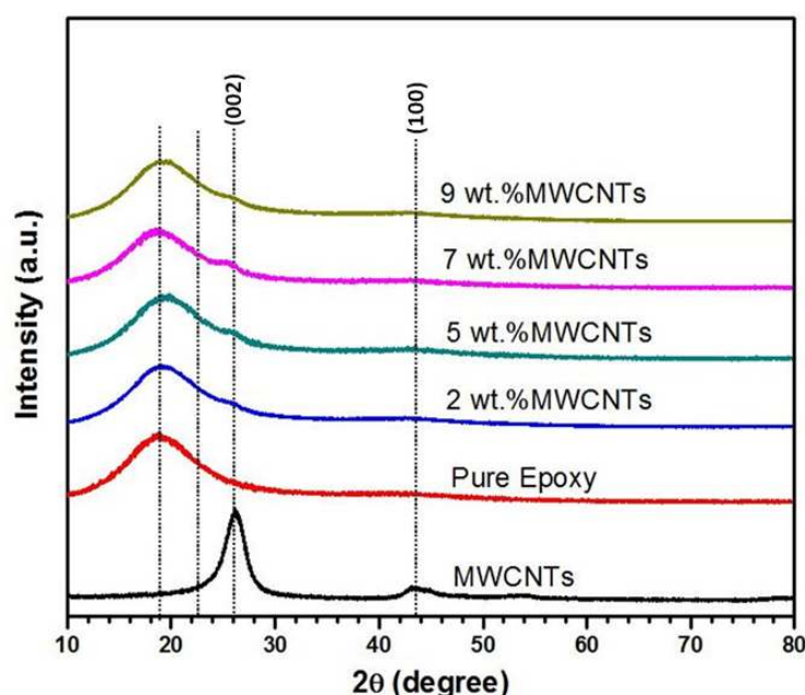
Fig. 2. XRD patterns of MWCNTs, pure epoxy and MWCNTs-epoxy composites
