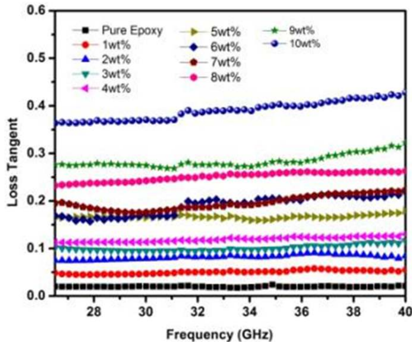
Fig. 4. Dielectric loss tangents of pure epoxy and MWCNTs-epoxy samples with MWCNT loading fractions from 1 – 10 wt.%
