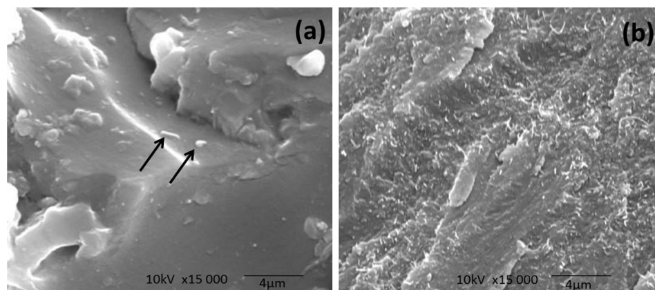
Fig. 1. SEM images of MWCNT-epoxy composite samples with the MWCNT loading of (a) 2 wt.% and (b) 9 wt.%. The black arrows in (a) points to dispersed MWCNTs in the epoxy matrix. MWCNTs are much more numerous and visible (everywhere) in the 9 wt.% sample as compared to the 2 wt.% one
