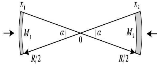
Fig. 2. Masses M_1 and M_2 in the form of ball segments with different thickness and matter density, located at the distance R from each other
