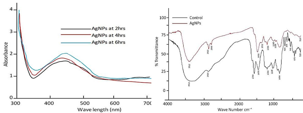
Fig. 1. Image showing the UV-visible and FTIR spectra obtained for the synthesized AgNPs. Left: UV spectra; Right: FTIR spectra observed for the synthesized AgNPs
