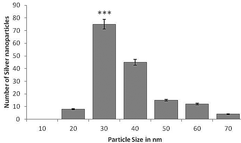
Fig. 3. Graph showing the total size distribution of synthesized AgNPs as viewed from SEM. All the values are average of triplicates and expressed as number \pm SD. *** Significant number observed ( p < 0.05 )
