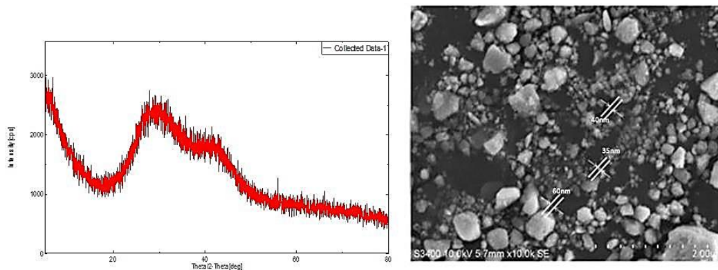
Fig. 2. Image showing the XRD spectra and SEM images of synthesized AgNPs. Left: XRD spectra. Right: HR-SEM analysis of synthesized AgNPs showing spherical shape and size of nanoparticles ranging between 30 – 60nm
