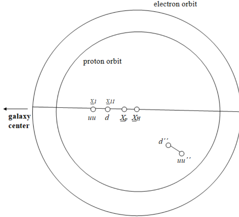
Fig. 2. Schematic structure of the test hydrogen atom in Figure 1 before and after a collision with another hydrogen atom in interstellar medium. The uu-d quarks before the collision have been moved to the positions denoted by uu''-d''
