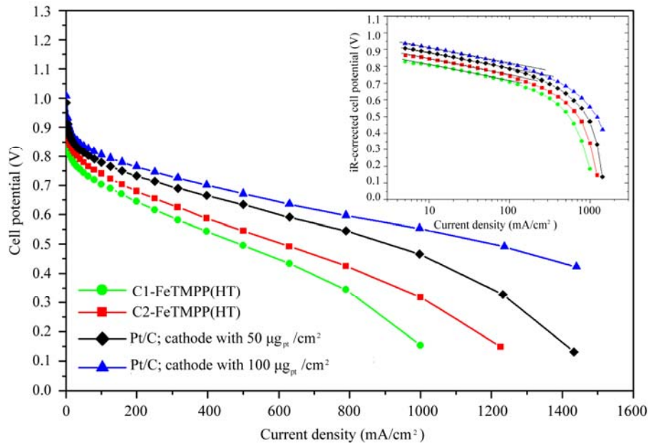
Figure 7. Single-cell PEMFC performance of C1-FeTMPP(HT), C2-FeTMPP(HT), and Pt/C oxygen reduction electrodes at 353 \text{ K} Anode: 0.4 \text{ mg}_{\text{Pt}}/\text{cm}^2 and cathode: 50 \text{ } \mu\text{g}_{\text{Fe}}/\text{cm}^2 . For comparison, performance of Pt/C as cathode with 50 or 100 \text{ } \mu\text{g}_{\text{Pt}}/\text{cm}^2 also shown. Inset shows the Tafel plots for the catalysts.
